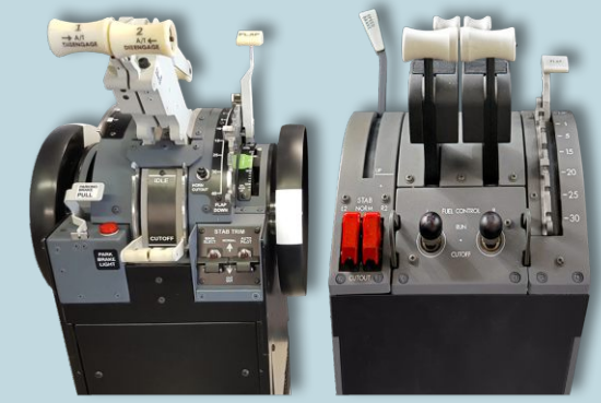
Simulated Boeing 737NG and 787 Throttles
